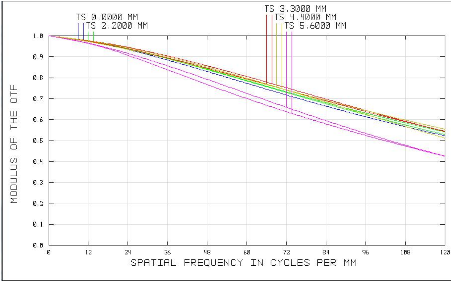
POLYCHROMATIC DIFFRACTION MTF
