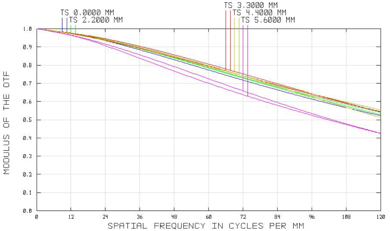
MTF(Frequency)
